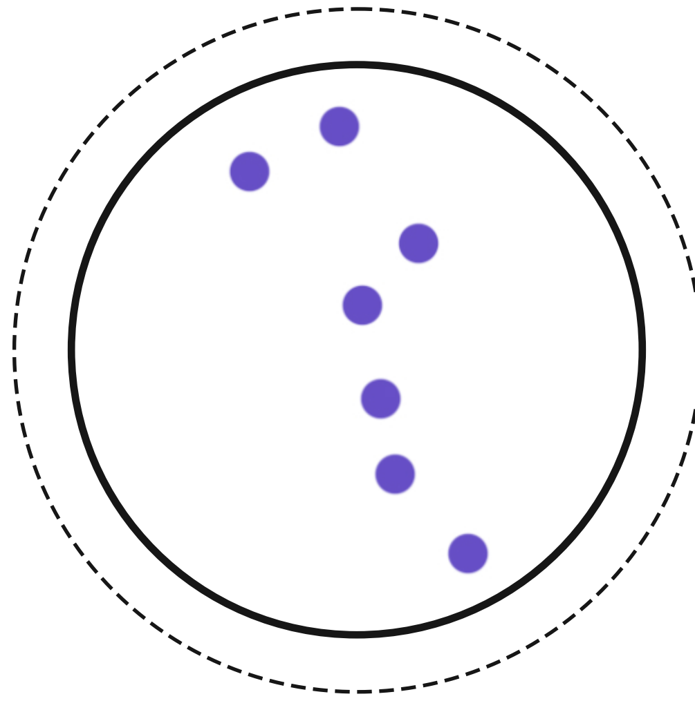
URSA MAJOR THE GREAT BEAR
