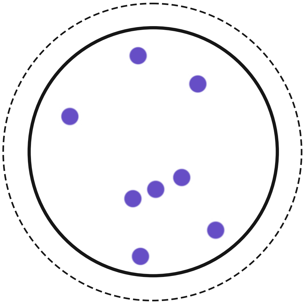
ORION THE HUNTER
